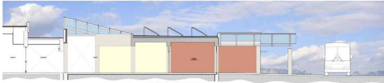
PROPOSED ATRIUM SECTION SCALE: 1/4" = 1'-0"
